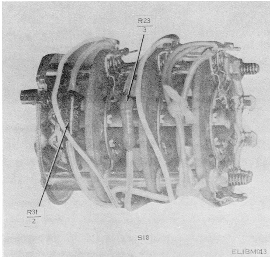
Figure 10. Switch assemblies (Sheet 2 of 4).
