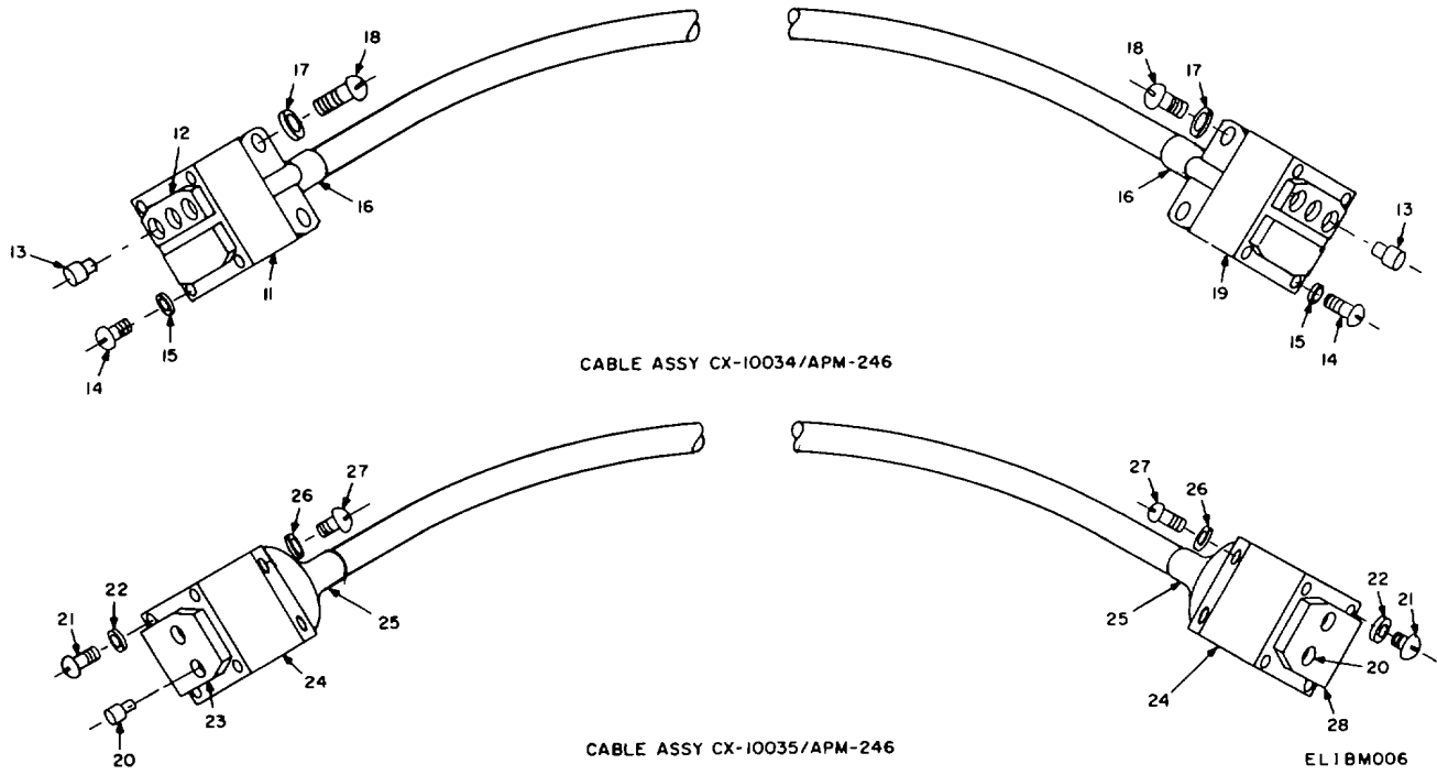
Figure 5, Cable Assemblies for AN/APM-246 (Sheet 2 of 2).
