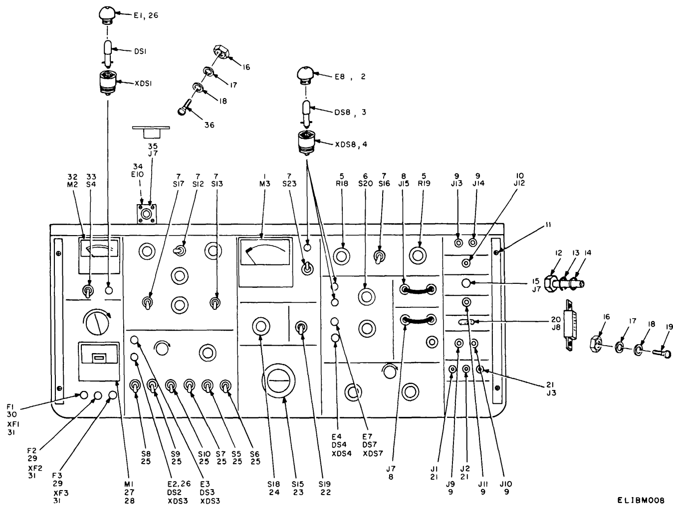
Figure 7. Test Set, Radar TS-2081 ( )/APM-247, front ( Sheet 1 of 2 ).
