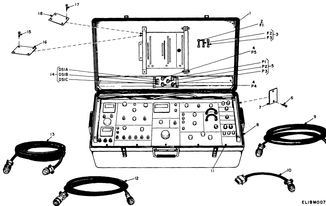
Figure 6. Test Set, Radar AN/APM-247.
