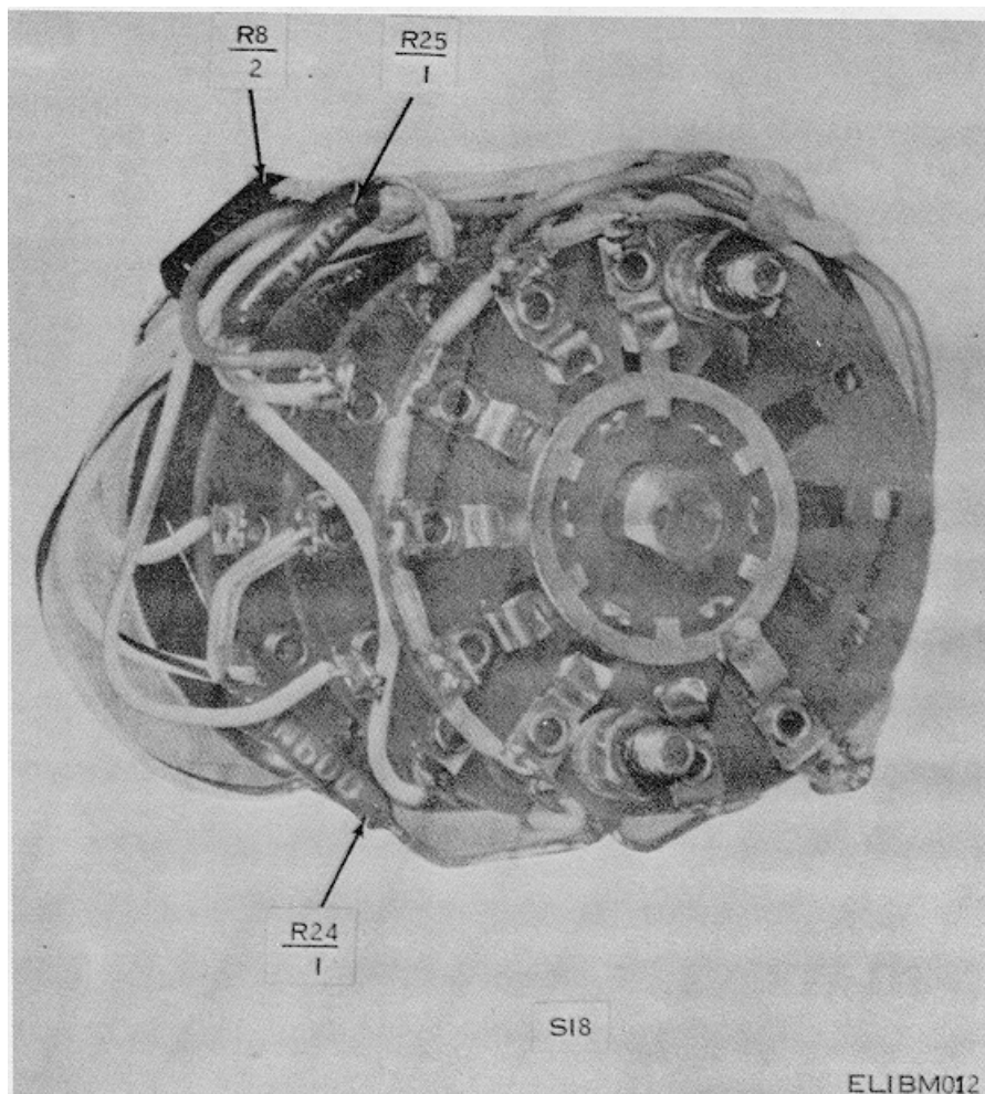
Figure 10. Switch assemblies (Sheet 1 of 4)
