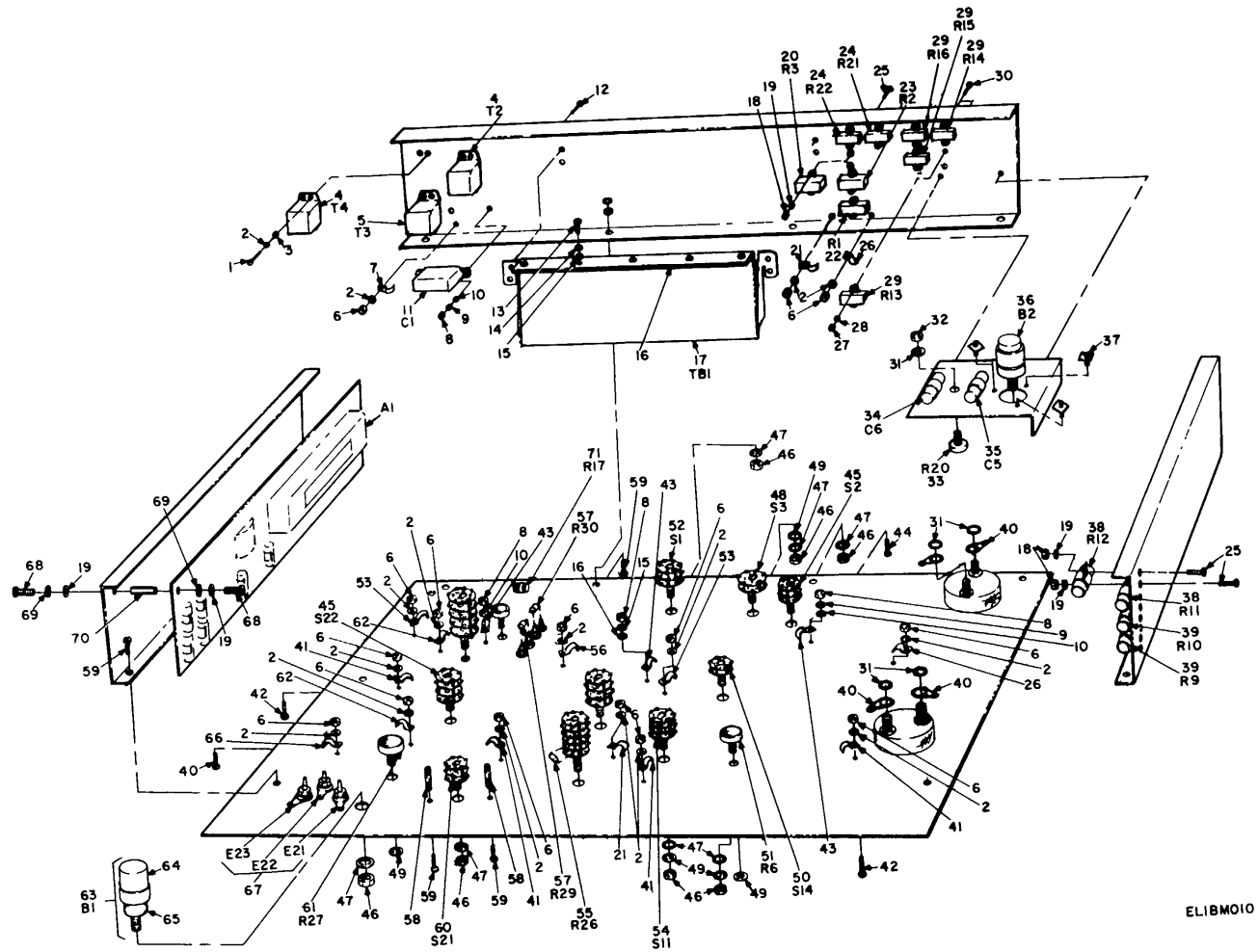
Figure 8. Test Set, Radar TS-2081 ( )/APM-247, internal view.
