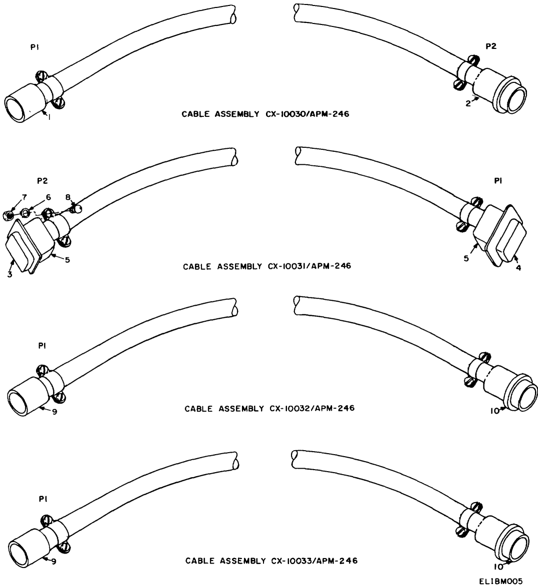
Figure 5. Cable Assemblies for AN/APM-246 (/SGEET 1 OF 2).
