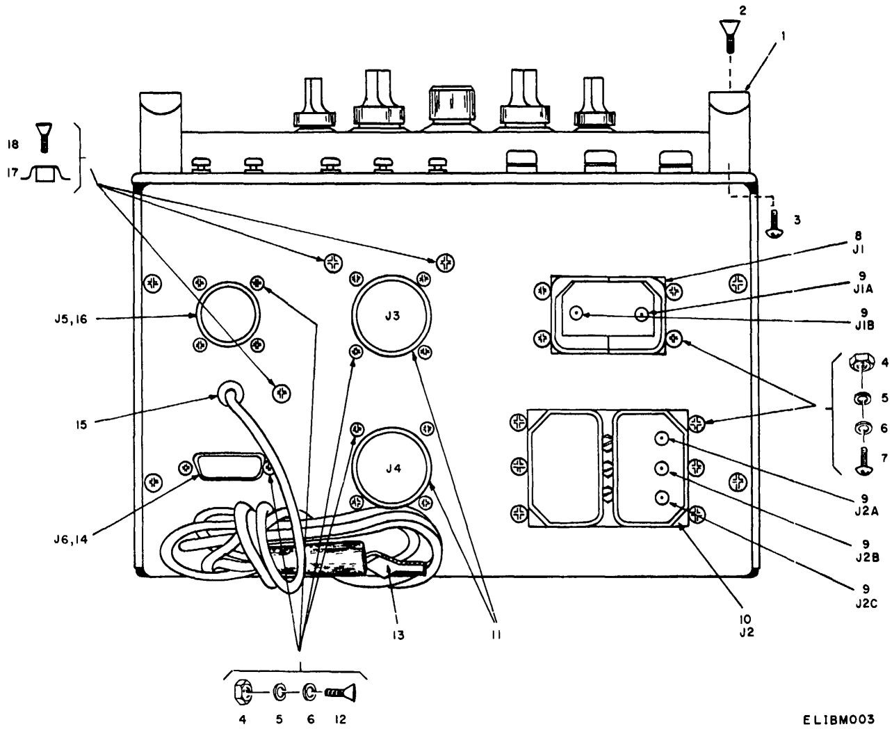
Figure 3. Test Set, Radar, Preflight TS-2154 ( ) /APM-246, rear.
