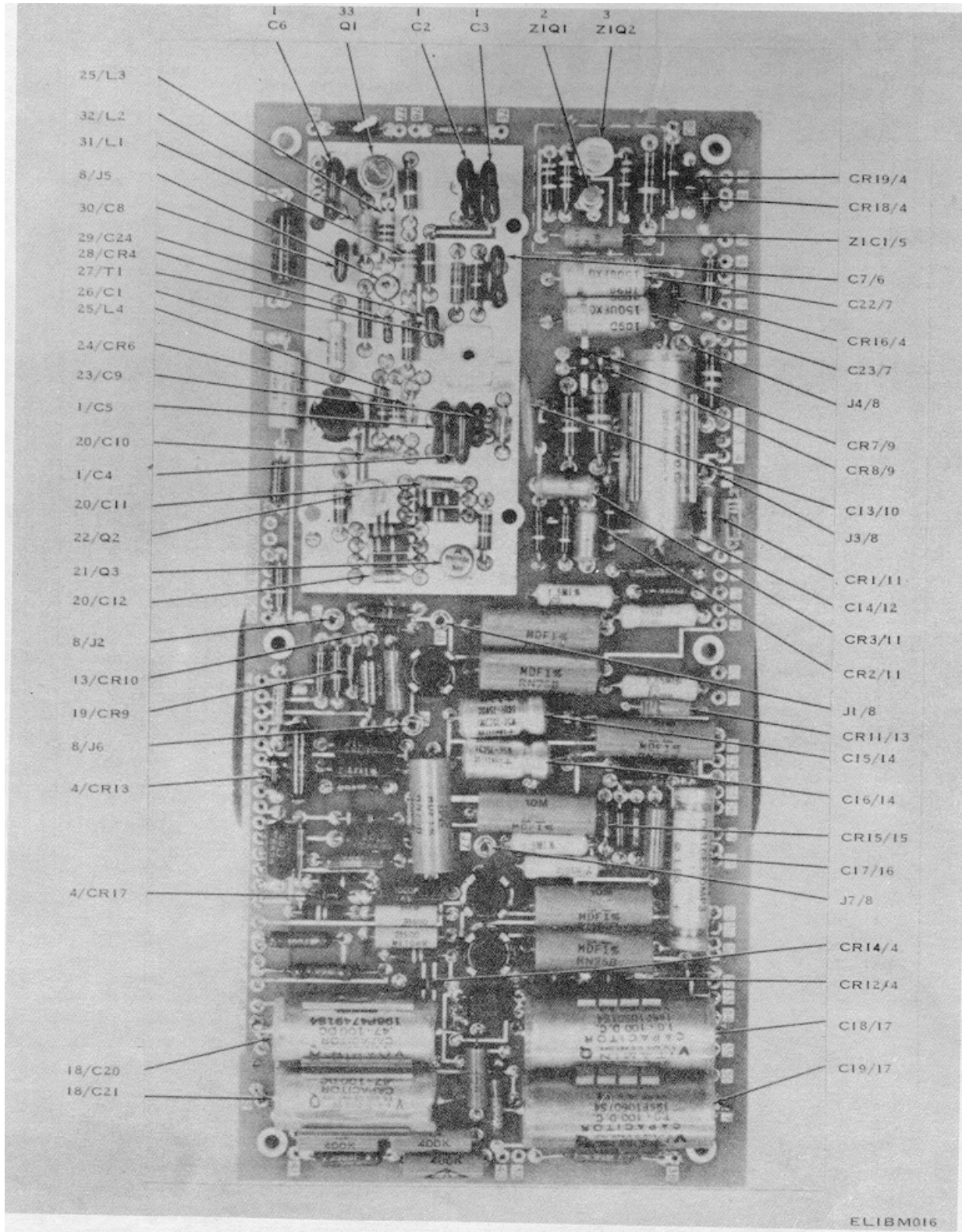
Figure 11. Printed circuit board (Sheet I of 2).
