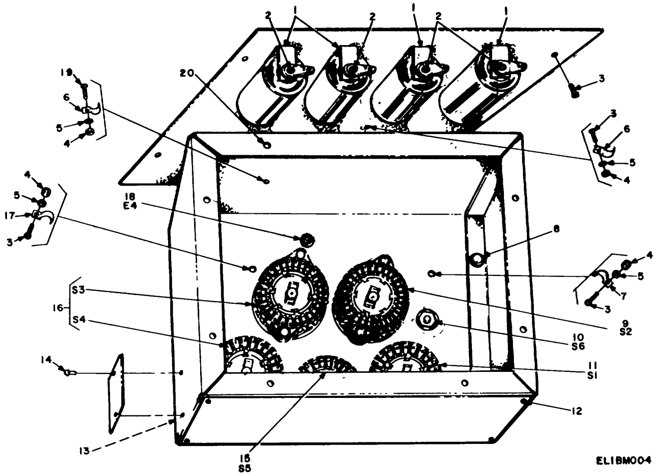
Figure 4. Test set, Radar, Preflight TS-2154 ( )/APM-246, bottom.
